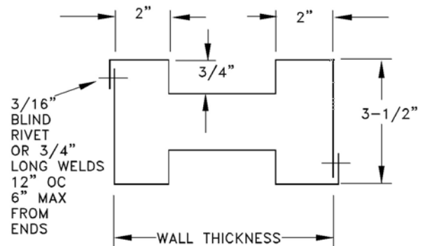
MULLION CROSS SECTION 16 GA. GALVANIZED STEEL
