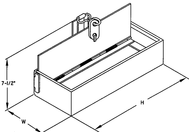
MODEL CRD50-6X SINGLE BLADE DAMPER
