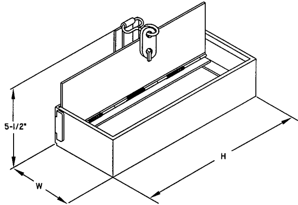
MODEL CRD50-4X SINGLE BLADE DAMPER
