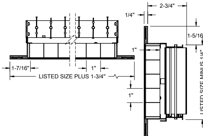
MODEL - WGAG100 - OPPOSED BLADE DAMPER
