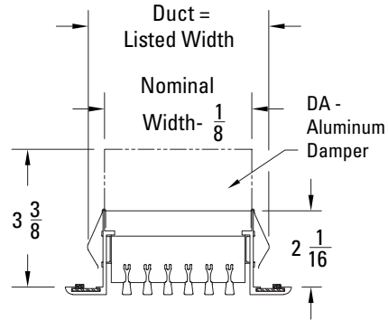
Option: DA Damper (2000 F)
