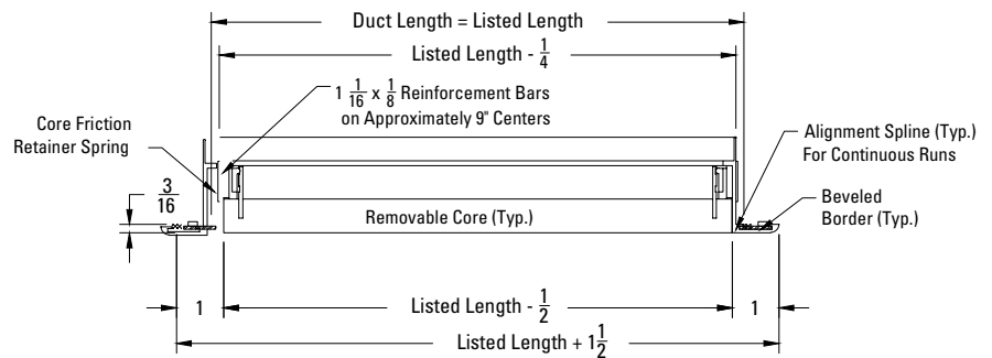
Side View (2000F)
