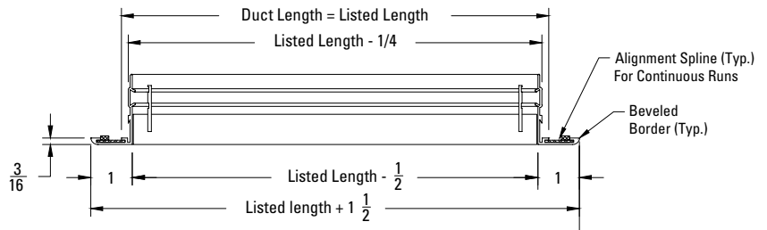
Side View (2000H & 2015H)
