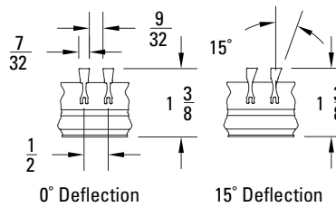
Option: 0° or 15° Deflection
