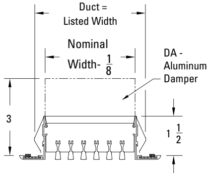
Option: DA Damper (2000 & 2015)
