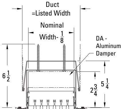
Option: DA Damper (2000 H & 2015 H)
