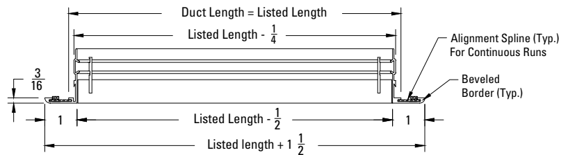
Side View (2000F)
