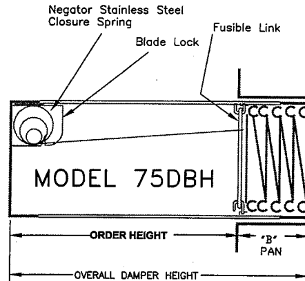
(H) HORIZONTAL MOUNT
