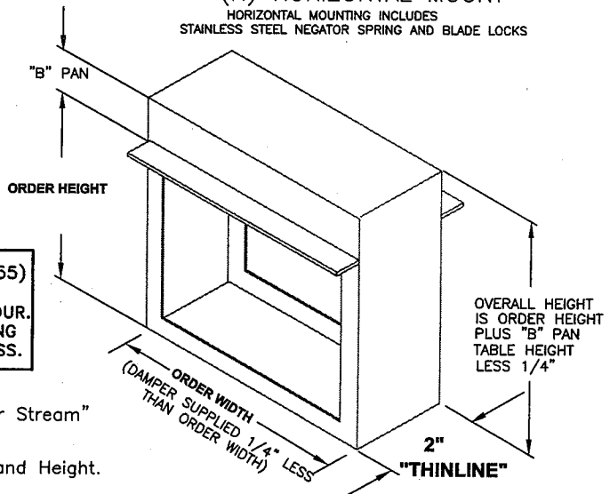
(H) HORIZONTAL MOUNT
