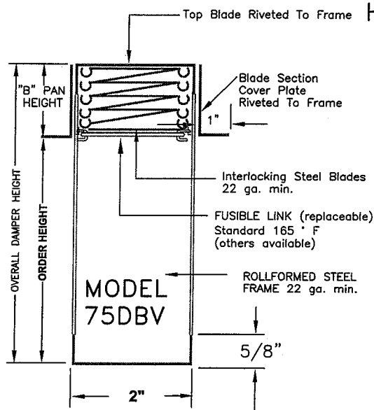
(V) VERTICAL MOUNT
