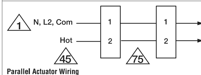
Parallel Actuator Wiring
